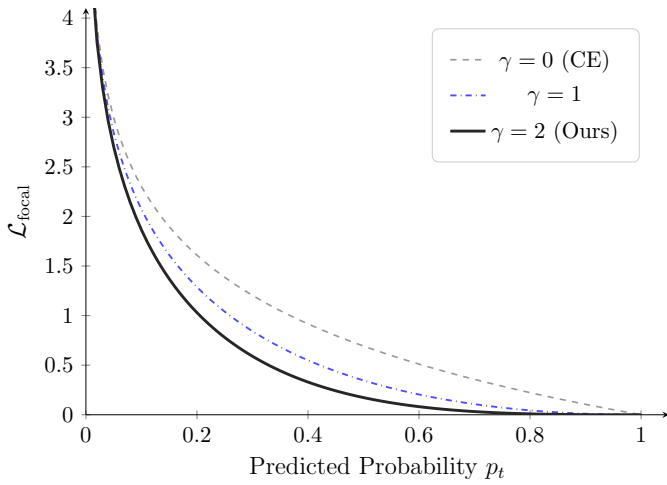
Focal Loss for Class Imbalance
