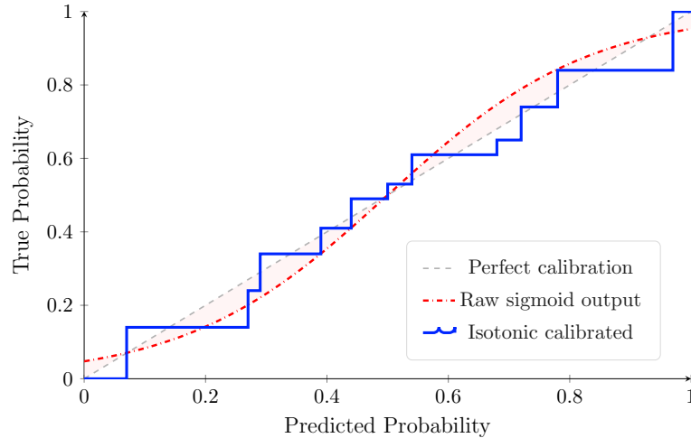
Isotonic Calibration of Meta-Learner
